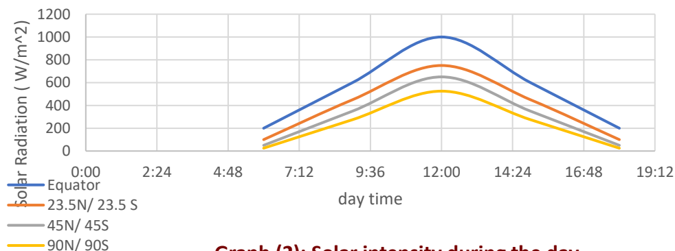
Graph (2): Solar intensity during the day
