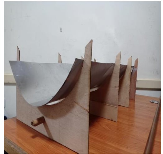
Figure (1): The prototype
